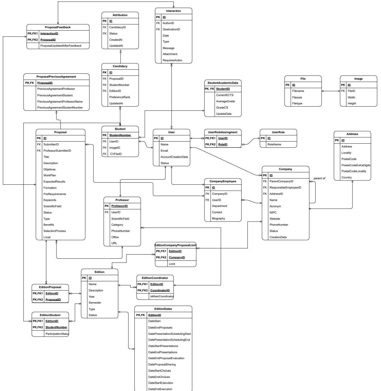
Figure D.1: Entity–Relationship Diagram, showing the main entities (users, students, professors, companies, editions, proposals, candidacies, and attributions) and their relationships
